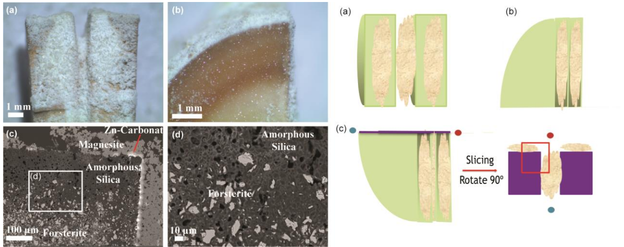
Figure 2.10 Optical photomicrograph of (a) the sample Fo100_f after reaction and (b) cross-section after cutting. The BSE images of (c) the edge of the Fo 100 _f and (d) the area that Fo 100 observed inside amorphous silica. Cartoon schematic for photo (a)-(c) of sample is shown in the right.
