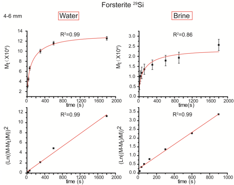
Figure 3.5 The exponential growth curve of the forsterite 29 Si NMR resonance from the 4-6 mm slice for the reactions in water and brine are shown. The semi-log plot of the same data is also displayed for reference. The 29 Si T 1 values extracted from the stretched exponential plots are 136 s for water and 153 s for the brine. The values from the semi-log plots are 159 s (± 8 s) for water and 289 s (± 11 s) for brine.
