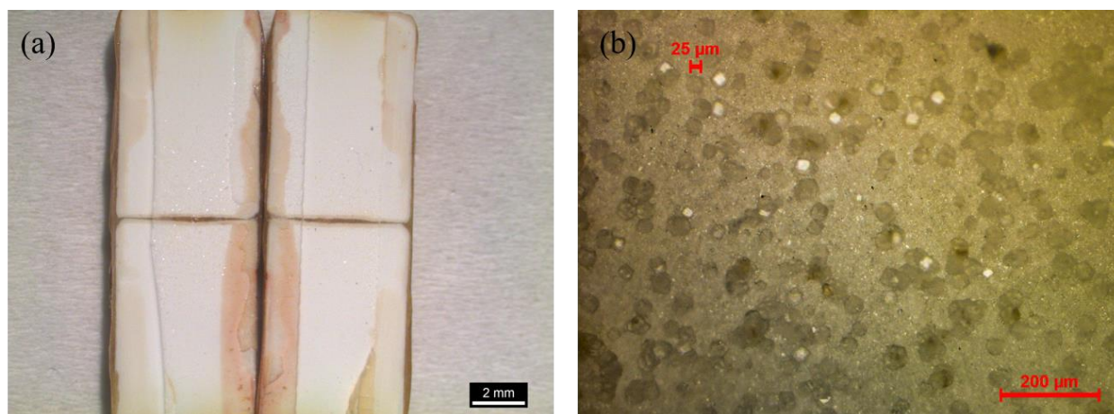
Figure 2.15 (a) Photo of sample Fo 100_fr , the forsterite monolith sample after the reaction (38 days) in water and ^{13}\text{CO}_2 . (b) Microscope image: solid-state carbonate crystals found on the fracture surface of this forsterite sample.
