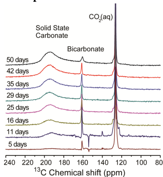
Figure 2.8 In-situ static ^{13}\text{C} NMR spectra of sample \text{Fo}_{100\_f} at different reaction times, held at 100\text{ }^\circ\text{C} and 100\text{ atm} ( ^{13}\text{CO}_2 pressure). A broad resonance consistent with solid-state carbonate formation (most evident peaked around 195\text{ ppm} ) grows in over time. Other resonances are \text{HCO}_3^- (aq) and \text{CO}_2 (aq).
