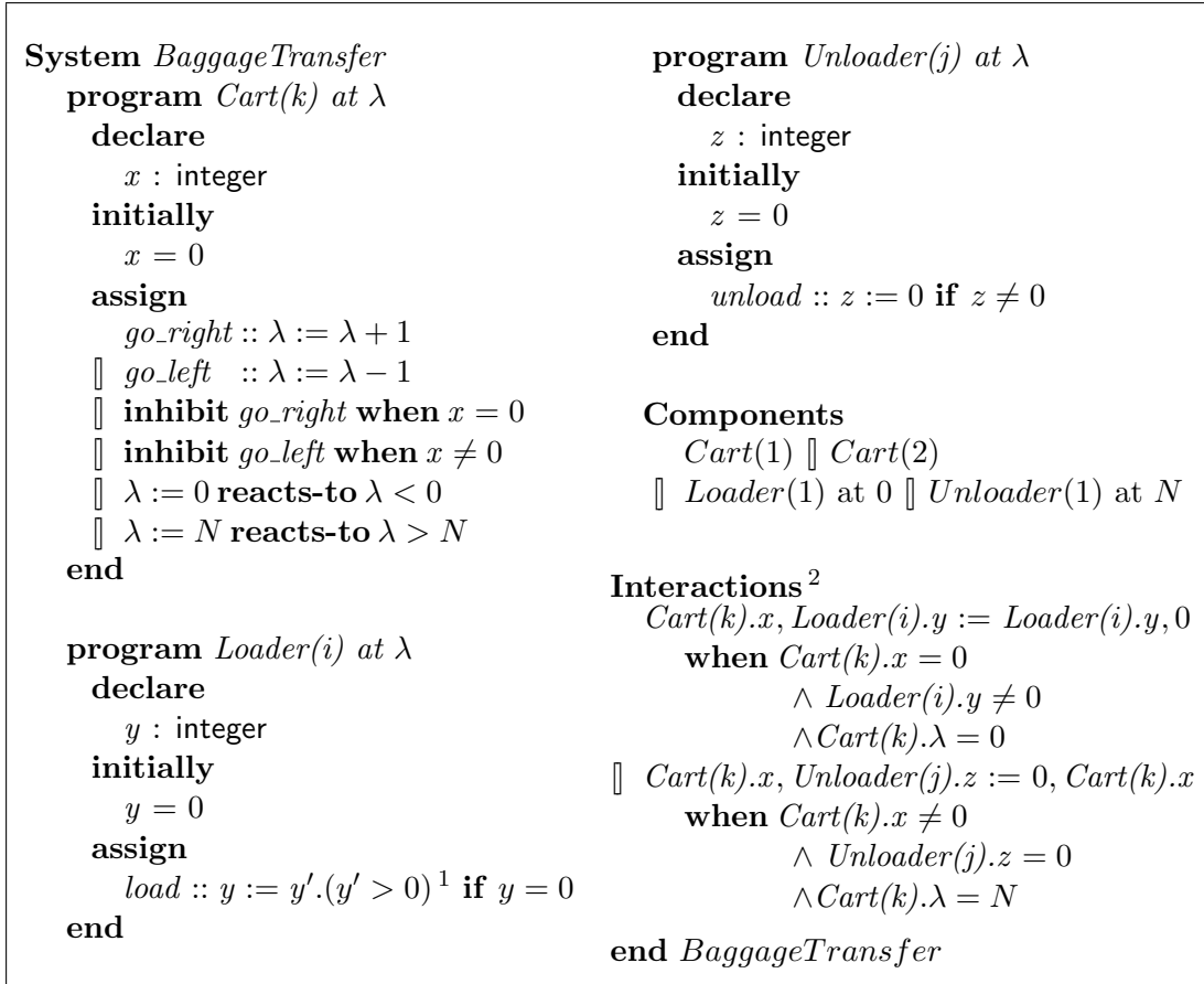
Fig. 1. An example Mobile UNITY system
