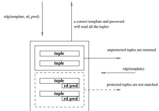
Figure 2: The execution of an rdg on a group of read-only and fully accessible tuples.
