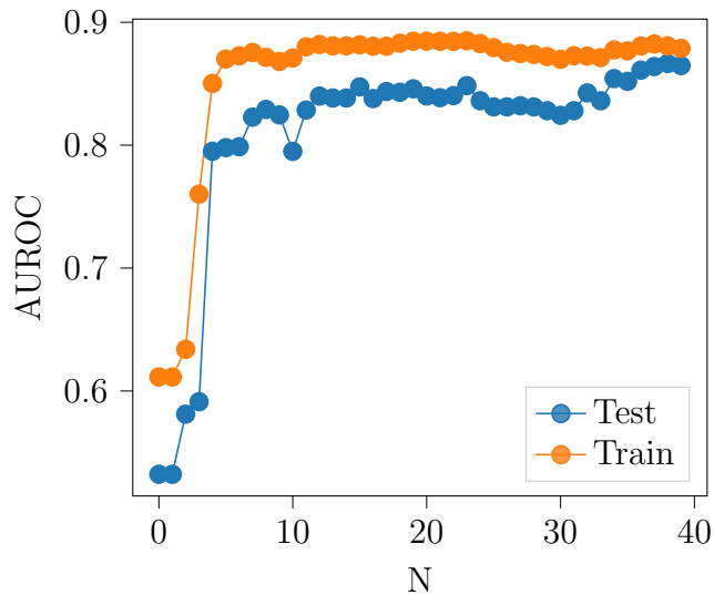
(a) AUROC
