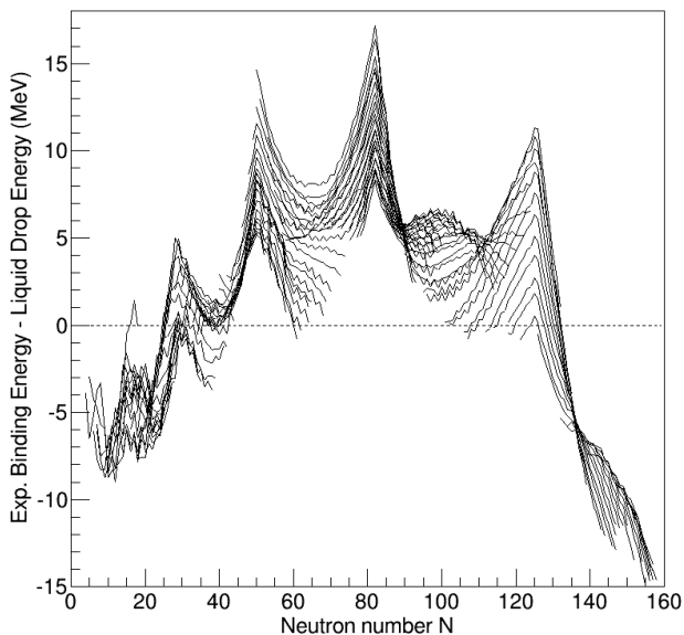
Figure 1.4: Residuals (experimental binding energy - LDM prediction) as a function of neutron number ( N ). Different curves correspond to different elements ( Z ). Large deviations from the data are seen at N = 28, 50, 82, and 126 . To keep these deviations in perspective, the total binding energies are roughly 8 \text{ MeV} \times the number of nucleons.
