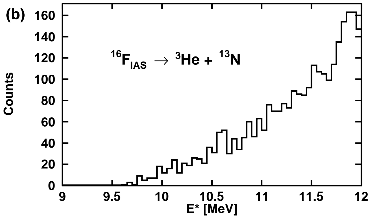
Figure 6.4: Excitation energy spectra for all detected (a) \alpha+^{12}\text{N} events and (b) ^3\text{He}+^{13}\text{N} events.
