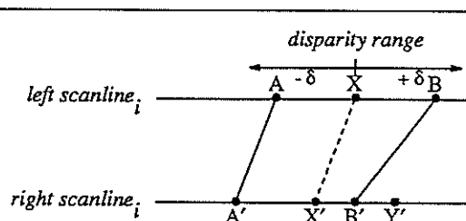
Figure 2. An intra-scanline ordering constraint.
