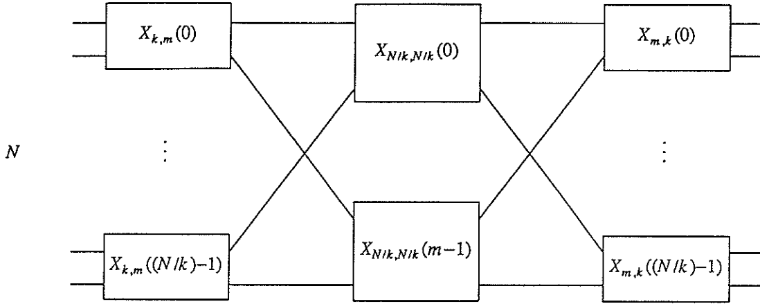
Figure 1: Clos Network
