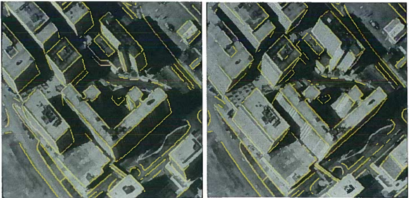
Fig. 6.2. Stereo aerial photographs over an urban area of Washington D.C. (All matched edgels are highlighted.)
