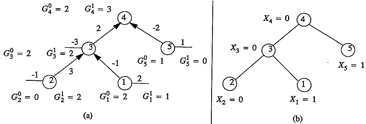
Figure 2: (a) Propagating goodness values, (b) Propagating activation values
