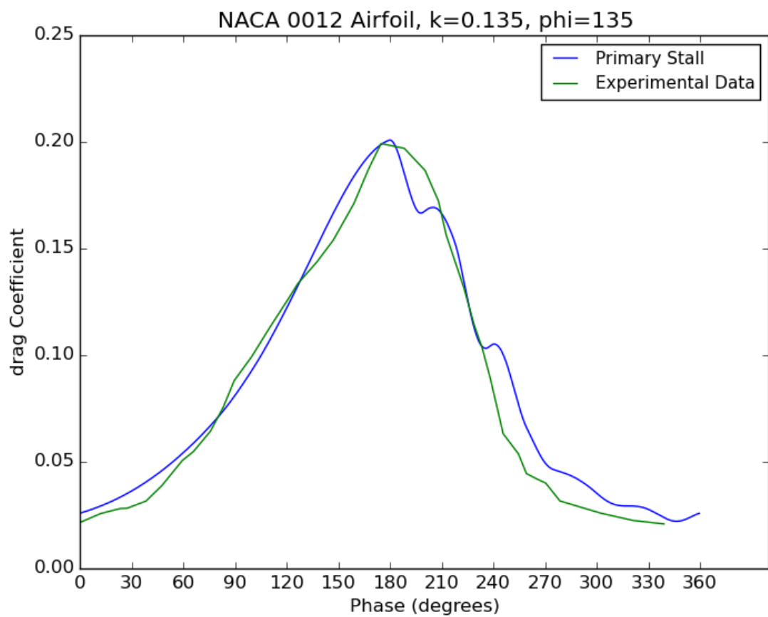
Figure 4.35 - Drag solutions for k=0.135 , compared to Ref [21]
