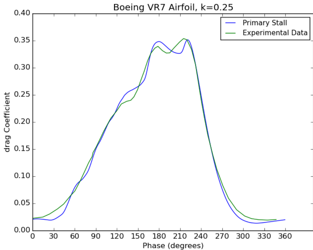
Figure 4.18 - Drag solutions for k=0.25 , compared to Ref [17]
