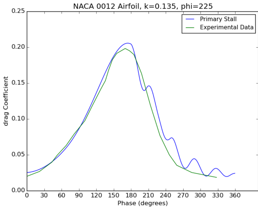
Figure 4.37 - Drag solutions for k=0.135 , compared to Ref [21]
