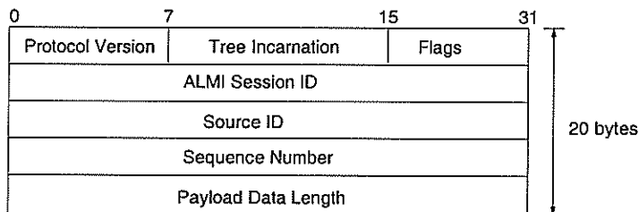
Figure 2: ALMI Packet Header Format
