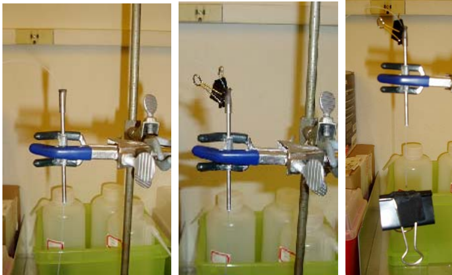
Figure A.8: Stand for suspending the fiber optic cable for flame cutting
