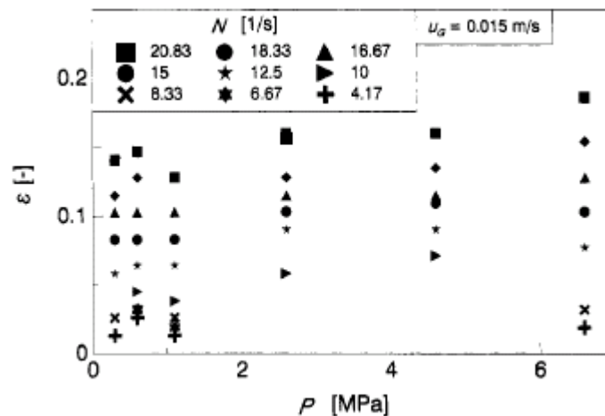
Figure 4.4: Effect of pressure on overall gas holdup (Source: Stegeman et al., 1995)
