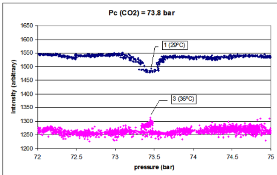
Figure 6.6: COP responses at the critical pressure boundary of \text{CO}_2
