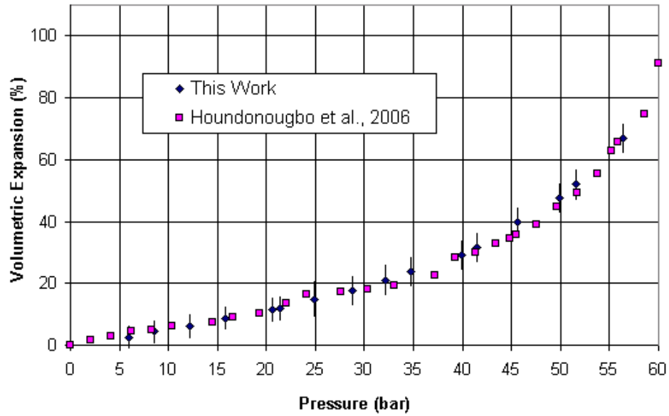
Figure B.2: Volumetric expansion of ethanol with CO 2 at 30 °C
