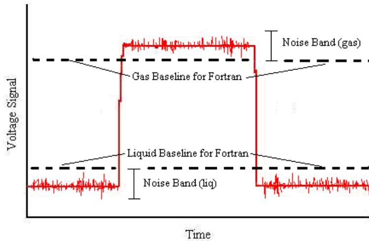
Figure A.24: Determination of gas and liquid baselines for processing
