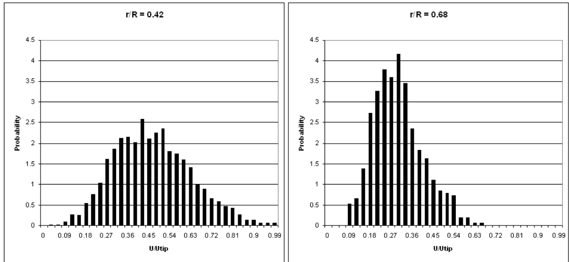
Figure 4.49: Change in mean radial velocity distribution with distance at 500 rpm and 12.5 L/min
