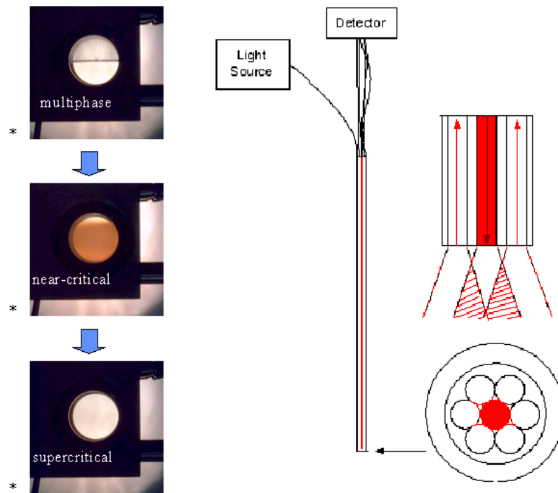
Figure 6.2: The critical opalescence probe/reflectometer (*Source: University of Leeds)
