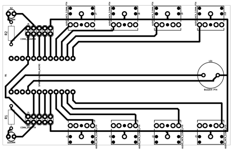
Figure 3 MEMS 312 PCB layout developed by Dr. Potter
