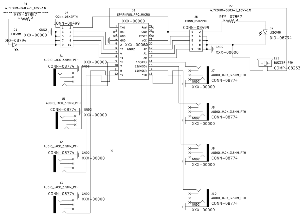
Figure 4 MEMS 312 PCB schematic
