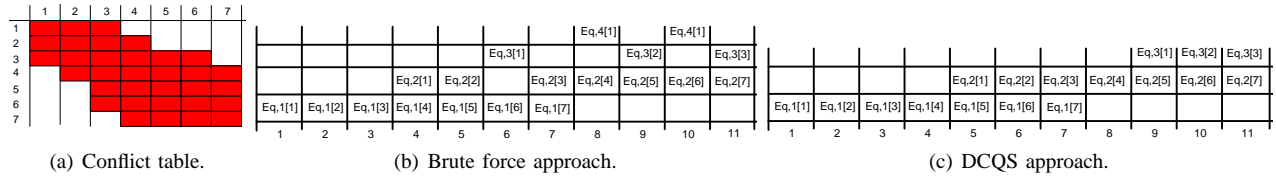
Fig. 3. Scheduling approaches.
